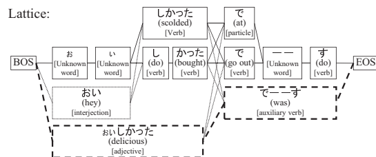
Figure 2: Example of a word lattice with new nodes “おい,” “おいしかった,” and “でーす.” The broken lines indicate the added nodes and paths, and the bold lines indicate the optimal path.
